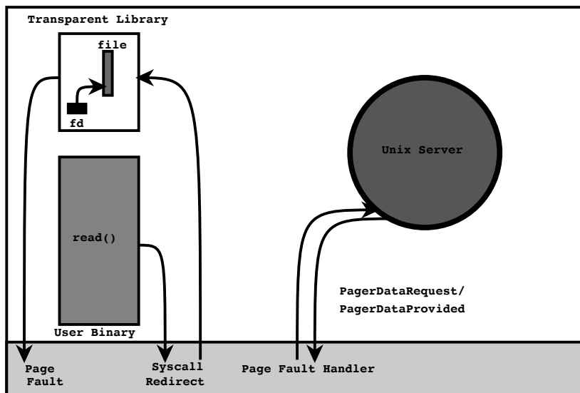
Figure 3-2: Implementation of Unix files as memory objects
