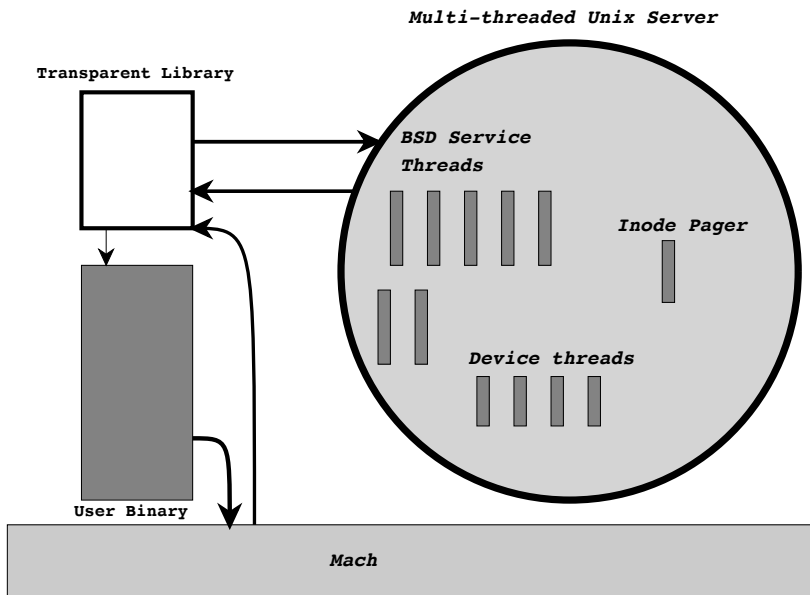
Figure 3-1: Organization of Unix services
